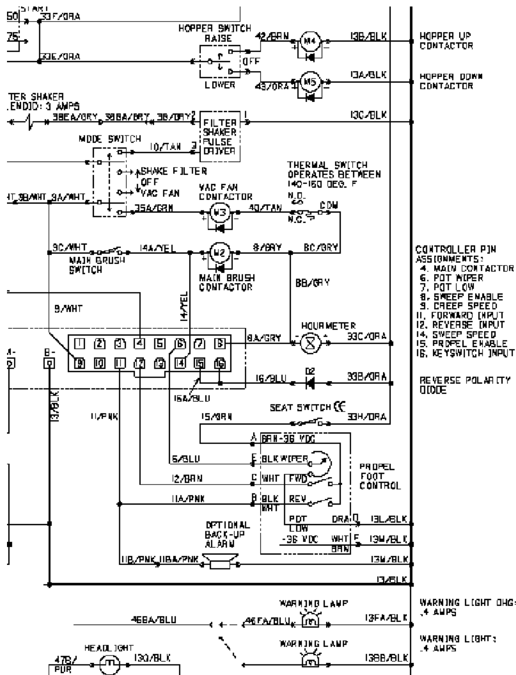
FIG. 2 - BACKUP ALARM KIT ELECTRICAL SCHEMATIC BILL OF MATERIALS FOR BACKUP ALARM KIT 384121
