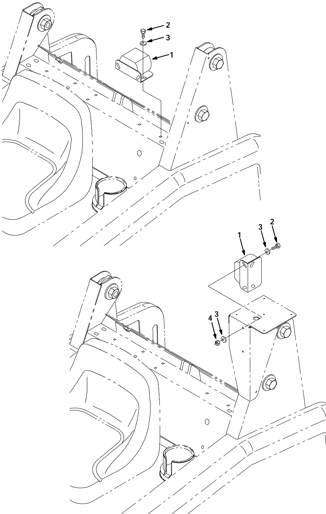
FIG. 1 - BACKUP ALARM KIT INSTALLATION
